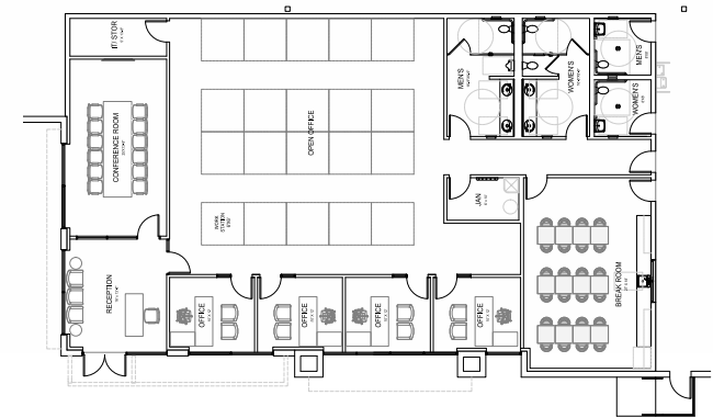
OFFICE PLAN
