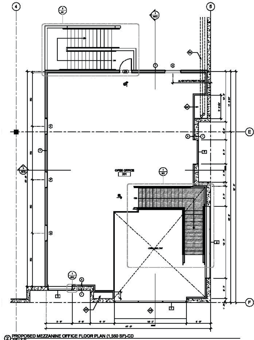
2 PROPOSED MEZZANINE OFFICE FLOOR PLAN (1,550 SF)-CD 1/4" = 1'-0"
